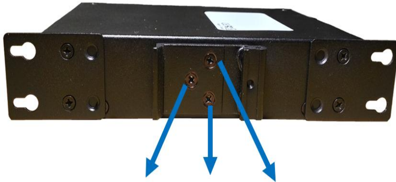
Figure 3.4: Remove DIN-Rail Bracket from the Switch
