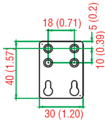
Figure 3.5: Wall Mounting Bracket Dimensions
