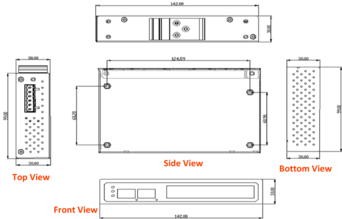
Figure 2.1: 065-7407GPOEP Physical Dimensions
